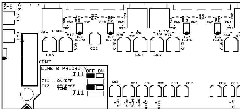
Location of CON7 on CX462
