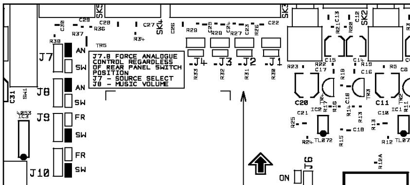
Location of Jumpers J1- 4 and J7- 10
